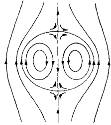
STEADY STREAMLINES DUE TO A VORTEX PAIR
